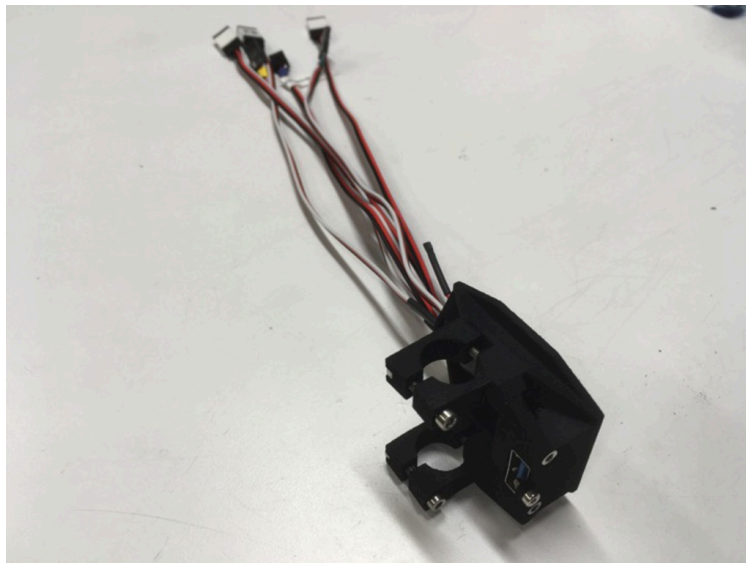
Figure 122: Interface cables for DJI.
