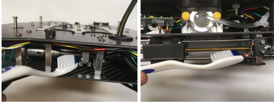
Figure 116: Left: Cleaning puncture leadscrew, located on the front of the system. Right: cleaning injection leadscrew, there are two of these one on each side of the system.
