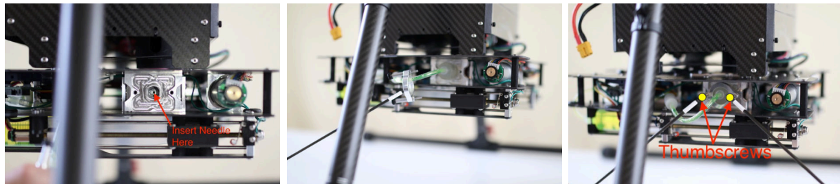
Figure 133: Left: Location to insert the needle. Center: Needle assembly holder. Right: Needle assembly holder in place.
