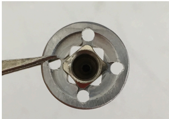
Figure 119: Needle tabs aligned with the cutouts on the retainer.
