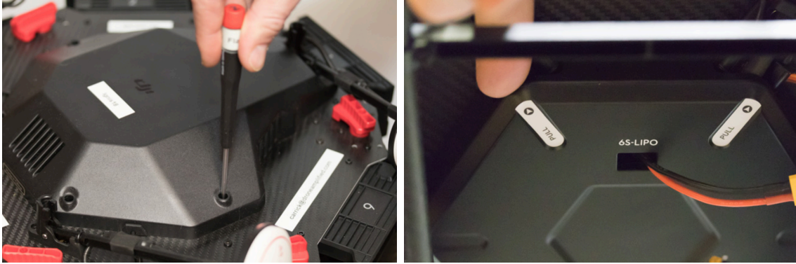
Figure 123: Unscrew top cover and remove bottom cover.
