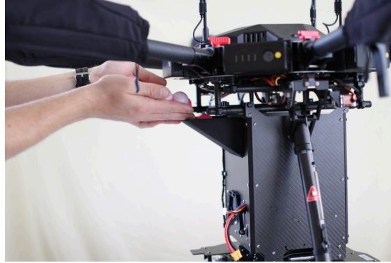
Figure 30: Filling the Hopper with ignition spheres.
