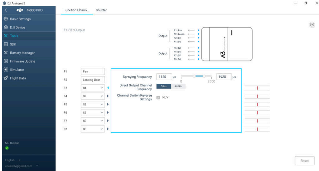
Figure 128: DJI Matrice 600 PWM Output Configuration.
