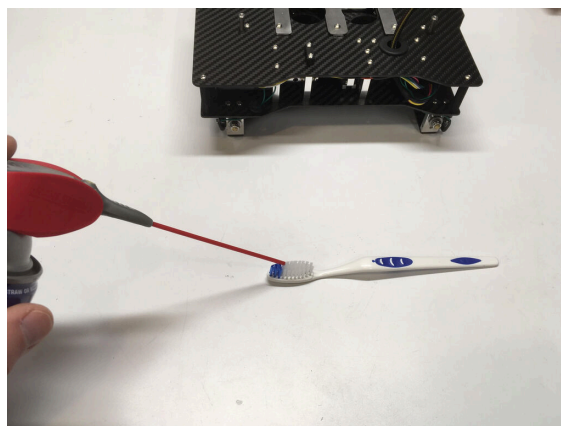
Figure 115: Apply a small amount of Graphite, Teflon or similar “dry” lubricant to the cleaning brush.
