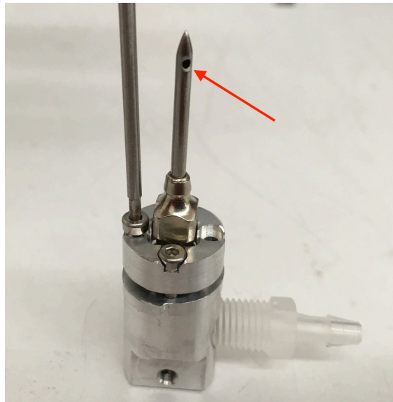
Figure 121: Needle hole oriented so that it will face downward when inserted in Ignis.
