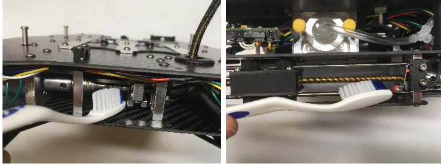
Figure 95: Left: Cleaning puncture leadscrew, located on the front of the system. Right: cleaning injection leadscrew, there are two of these one on each side of the system.
