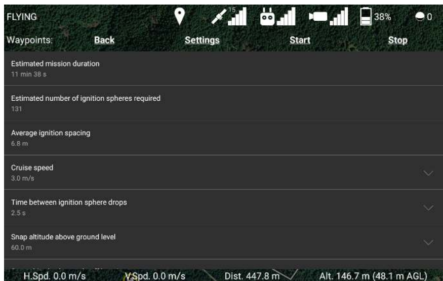
Figure 90: Setting up a waypoint mission with drop lines.
