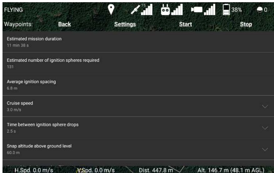
Figure 85: Waypoint mission settings.
