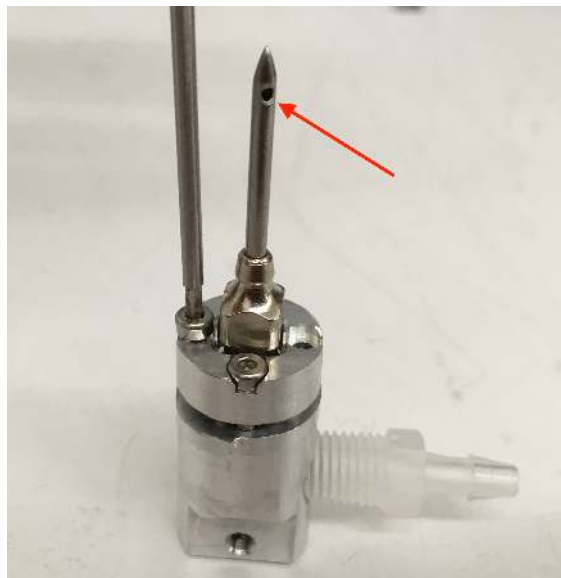
Figure 100: Needle hole oriented so that it will face downward when inserted in Ignis.
