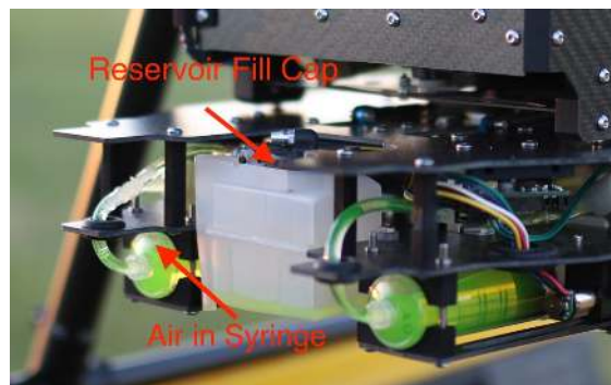
Figure 36: Reservoir fill location.
