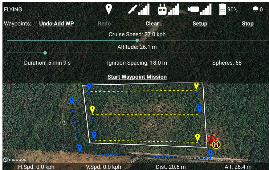
Figure 39: Setting up a waypoint mission with drop lines.
