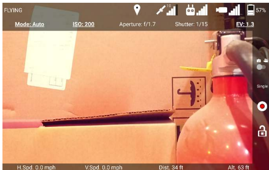
Figure 67: Exposure Menu
