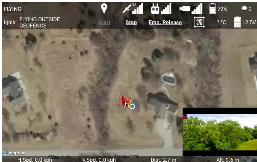
Figure 71: Ignis Menu
