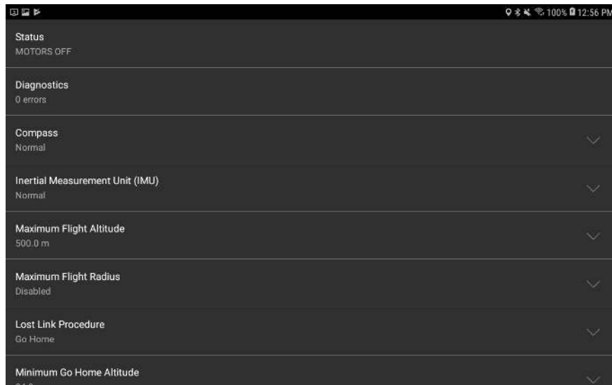
Figure 53: Drone Setup
