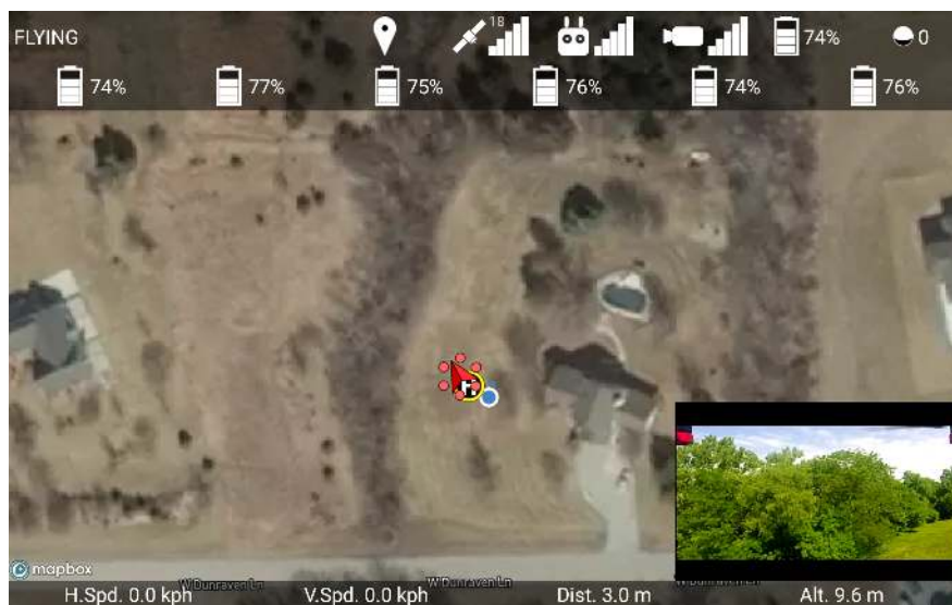
Figure 70: Battery Menu
