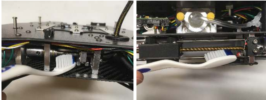
Figure 94: Left: Cleaning puncture leadscrew, located on the front of the system. Right: cleaning injection leadscrew, there are two of these one on each side of the system.
