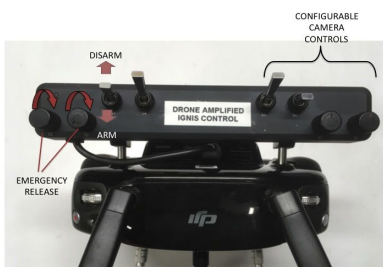
Manual trigger
